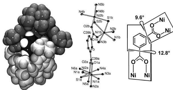
Figure 3. Left: van der Waals representation of the [(\text{LNi}^{\text{II}}_2)-(\mu\text{-isophthalato})]^{2+} dication in crystals of 4[\text{BPh}_4]_2 \cdot 4\text{MeCN} \cdot \text{EtOH} . Middle: ORTEP representation of the core structure of 4 with the atom labeling Scheme. Ellipsoids are represented at the 50% probability level. Right: Tilting of the \text{Ni}_2 carboxylato planes in 4 .
